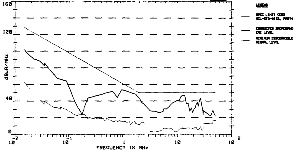
CONDUCTED BROADBAND EMISSIONS NEUTRAL LINE FIG 17 - STANDARD MODEL 1100 GRID COMPUTER CONDUCTED BROADBAND EMISSIONS (NEUTRAL LINE)
