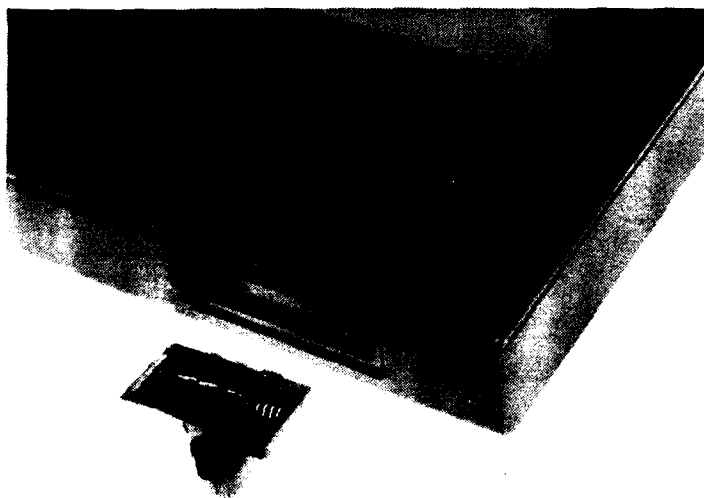
FIG 12 - DISPLAY LATCH FAILURE OF TEMPEST MODEL 1107 GRID COMPUTER FROM FREE FALL TEST DEF STAN 07-55 PART 2 SECTION 1/1 TEST A9
