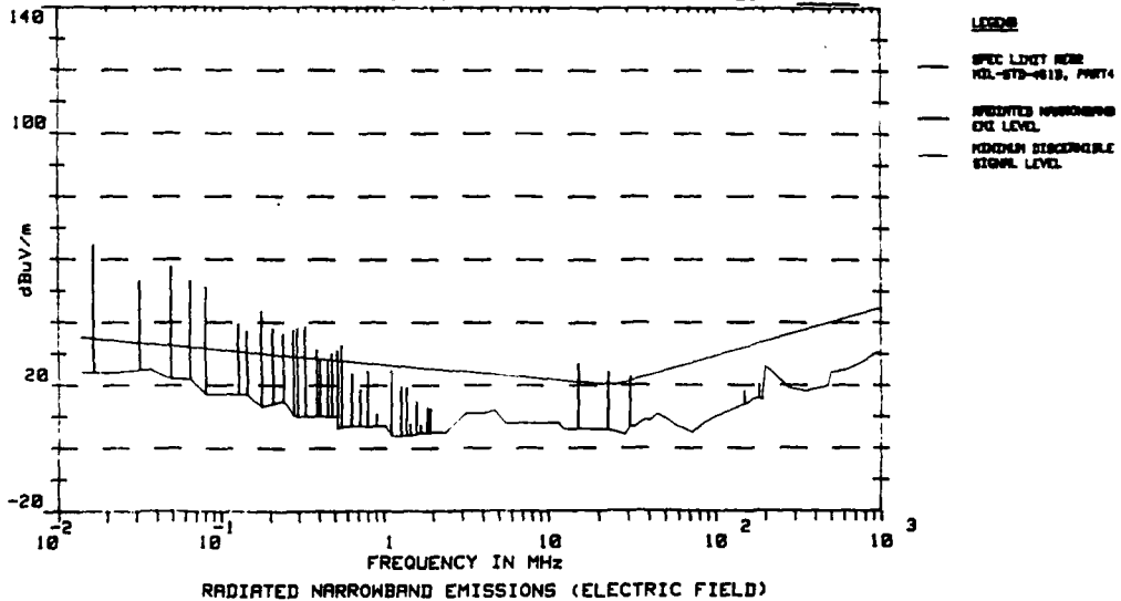
FIG 26 - TEMPEST MODEL 1107 GRID COMPUTER RADIATED NARROWBAND EMISSIONS (ELECTRIC) SERIAL CABLE DISCONNECTED
