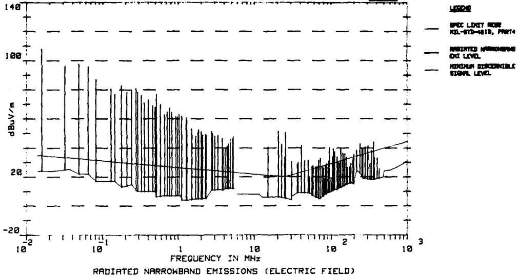
FIG 25 - STANDARD MODEL 1100 GRID COMPUTER RADIATED NARROWBAND EMISSIONS (ELECTRIC) SERIAL CABLE DISCONNECTED
