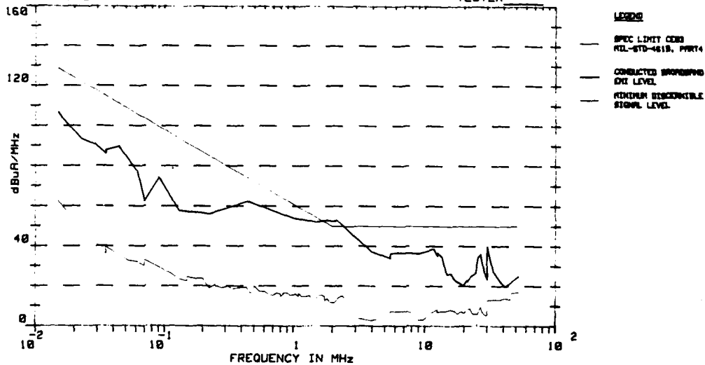
CONDUCTED BROADBAND EMISSIONS (NEUTRAL LINE) FIG 18 - TEMPEST MODEL 1107 GRID COMPUTER CONDUCTED BROADBAND EMISSIONS (NEUTRAL LINE)
