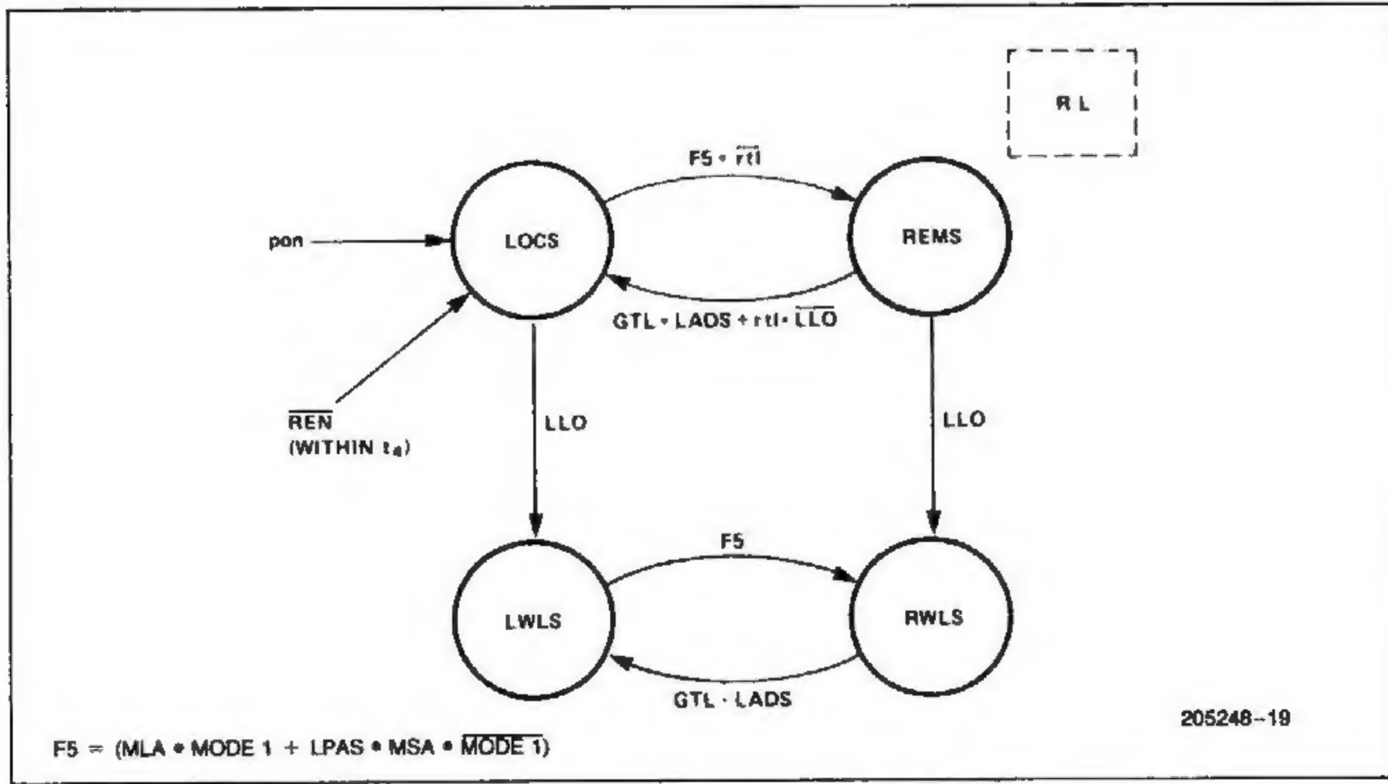
Figure A-1. 8291A State Diagrams (Continued)
