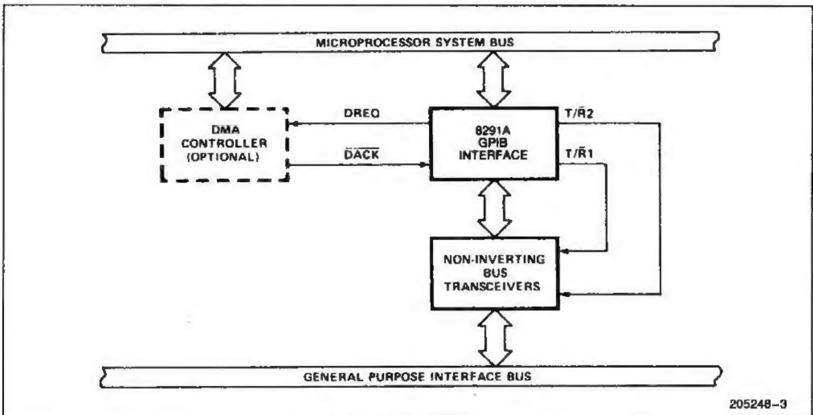
Figure 3. 8291A System Diagram
