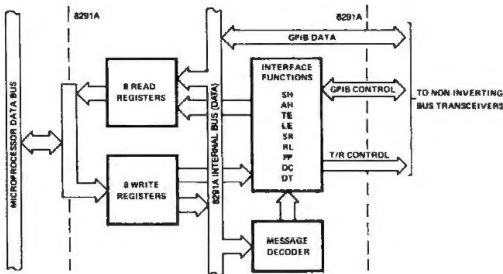
Figure 1. Block Diagram
