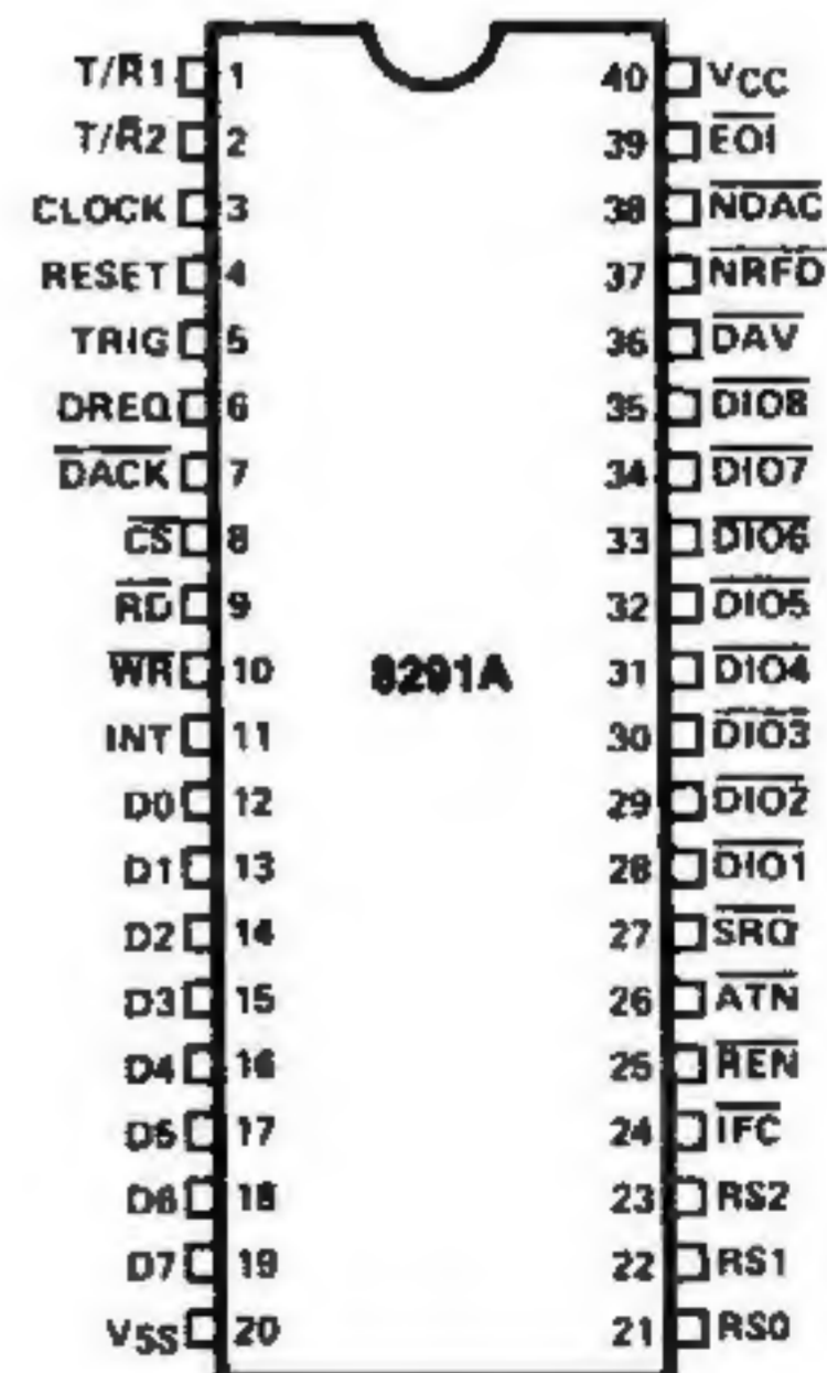
Figure 2. Pin Configuration
