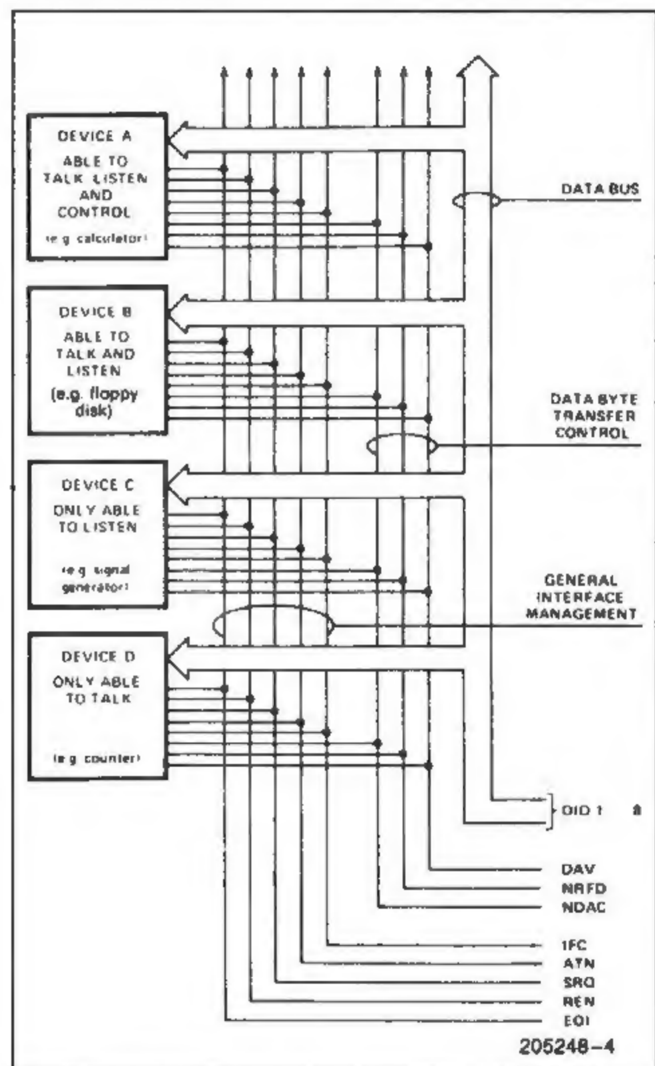
Figure 4. Interface Capabilities and Bus Structure
