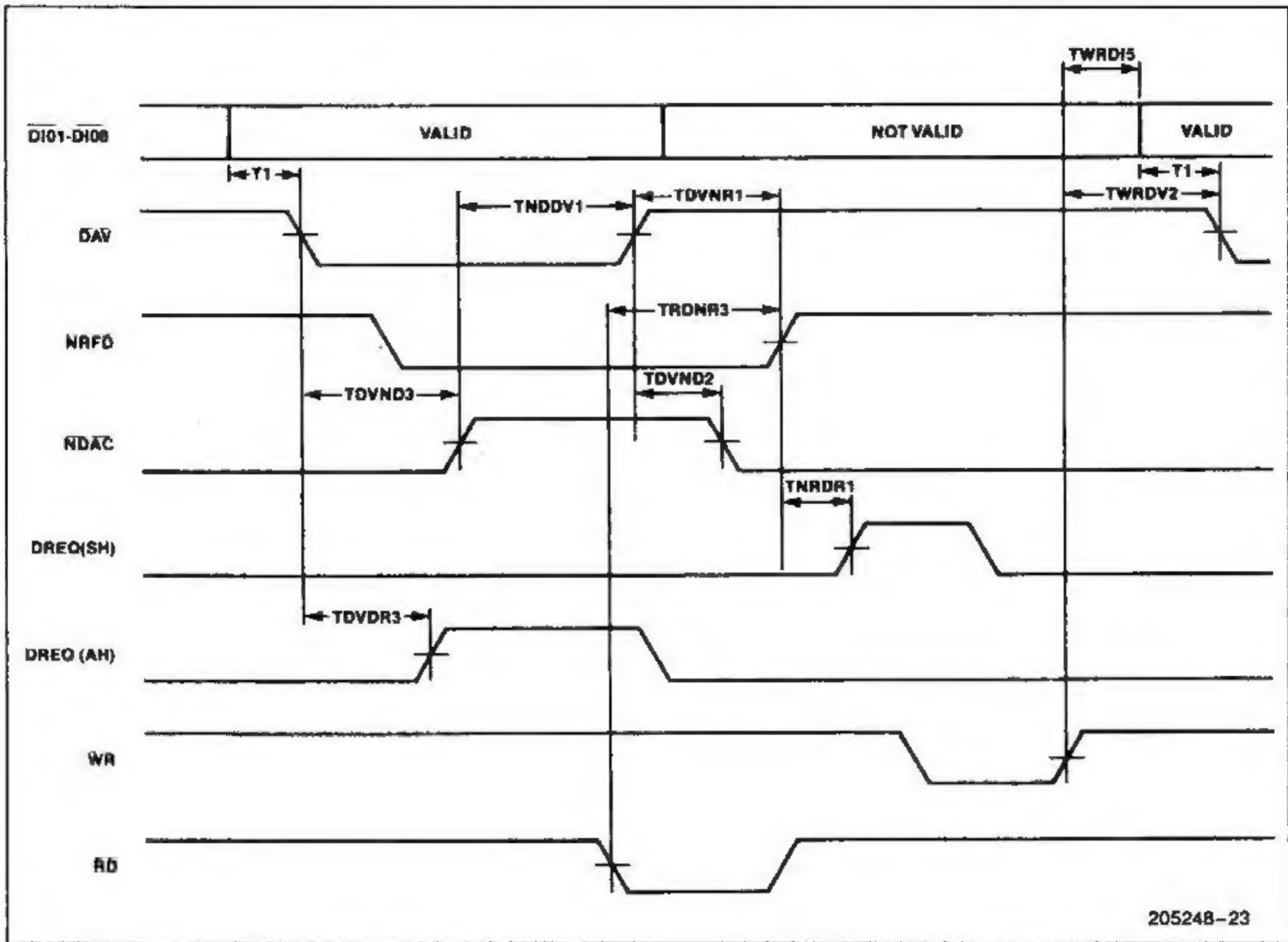
Figure C-1. 3-Wire Handshake Timing at 8291A
