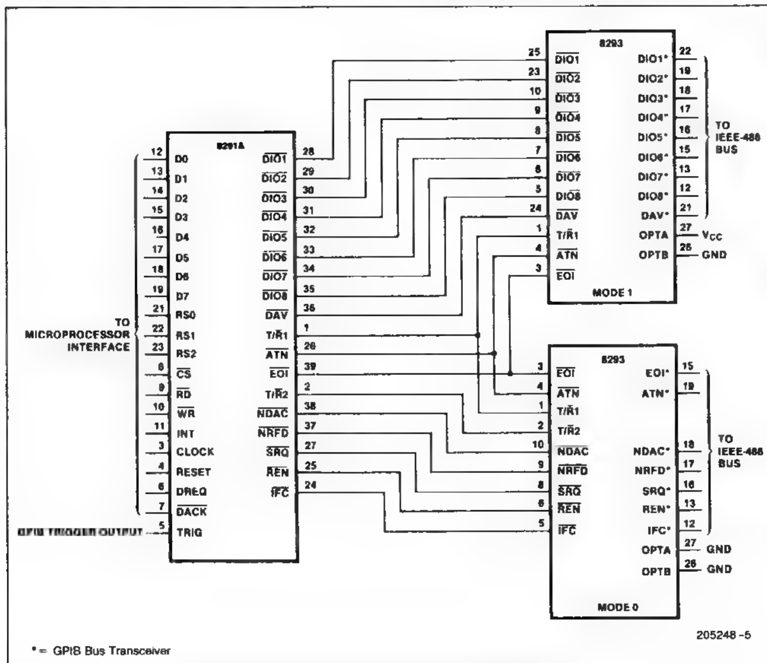
Figure 6. 8291A and 8293 System Configuration
