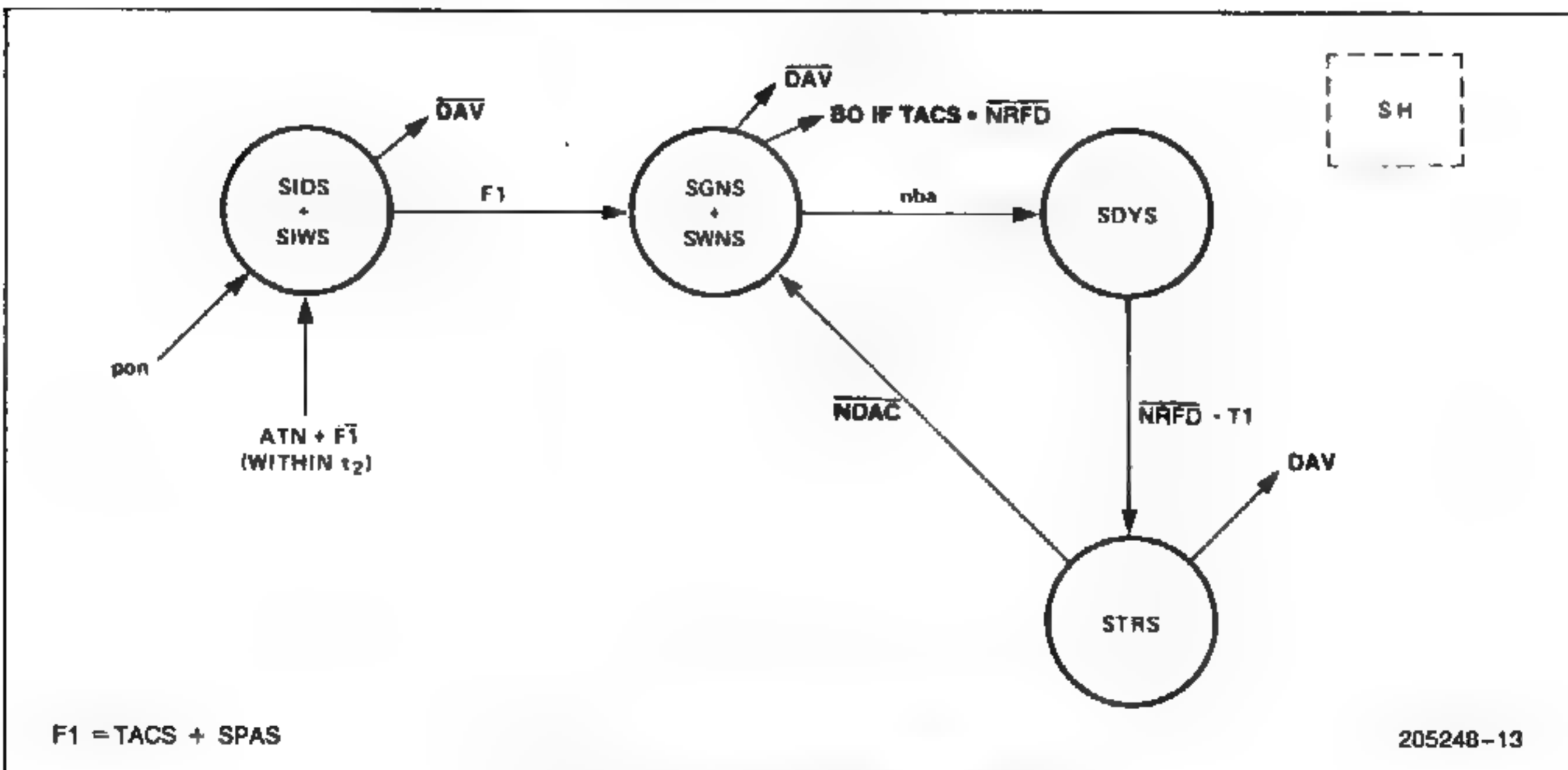
Figure A-1. 8291A State Diagrams
