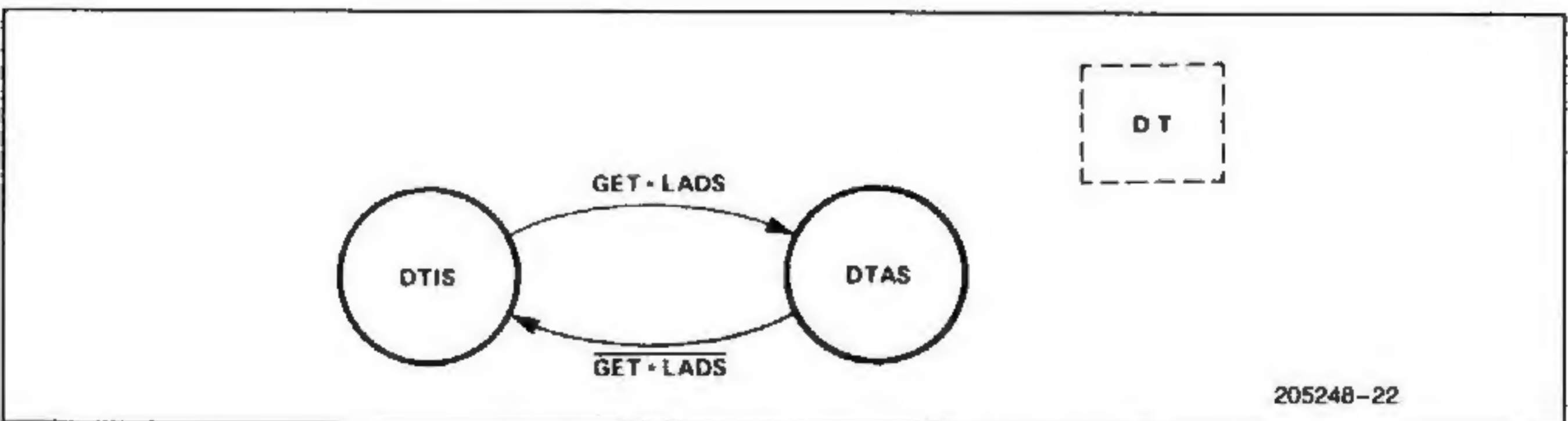
Figure A-1. 8291A State Diagrams (Continued)
