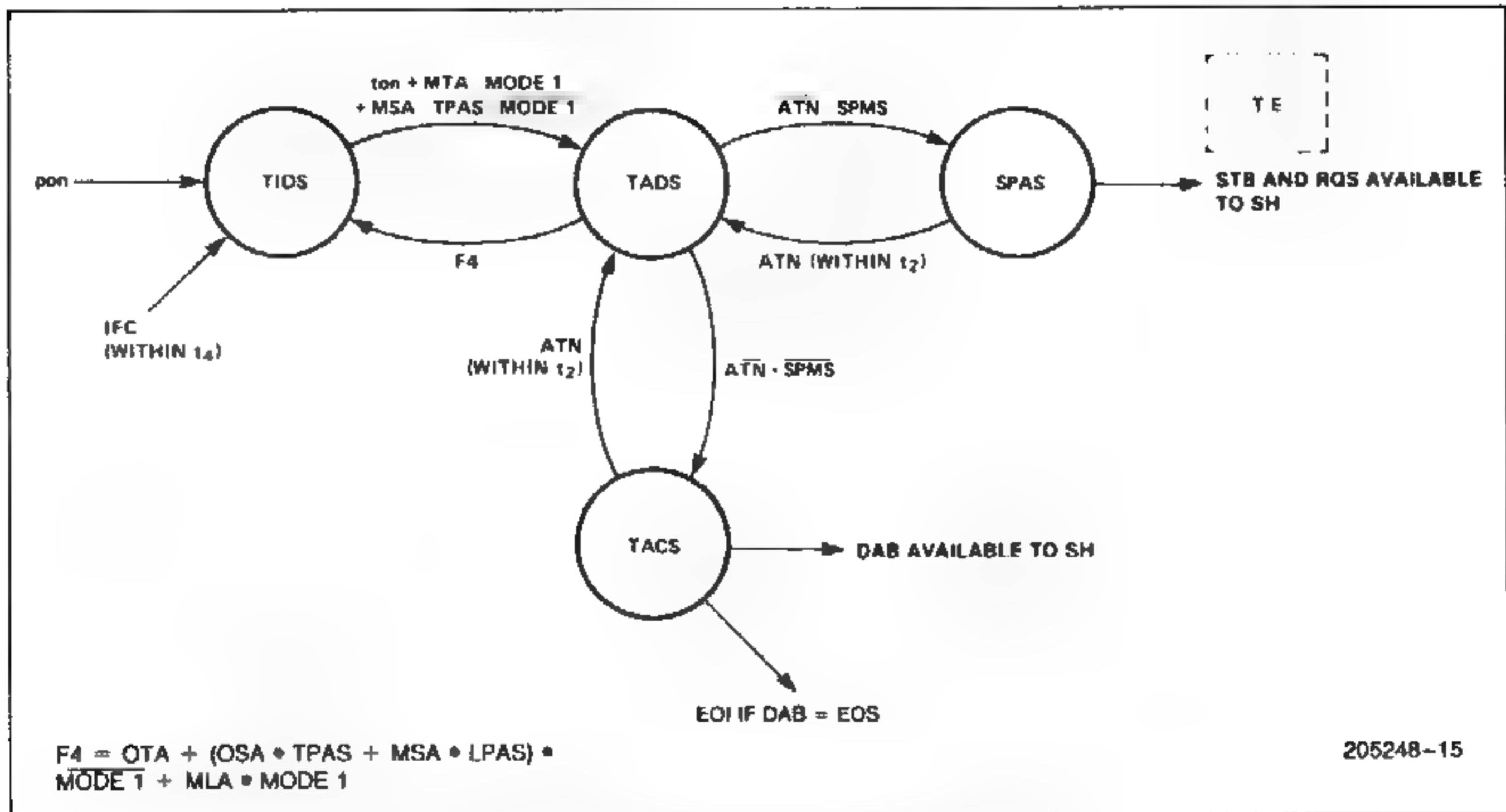
Figure A-1. 8291A State Diagrams (Continued)
